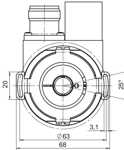
Flange type 3 with stator coupling
